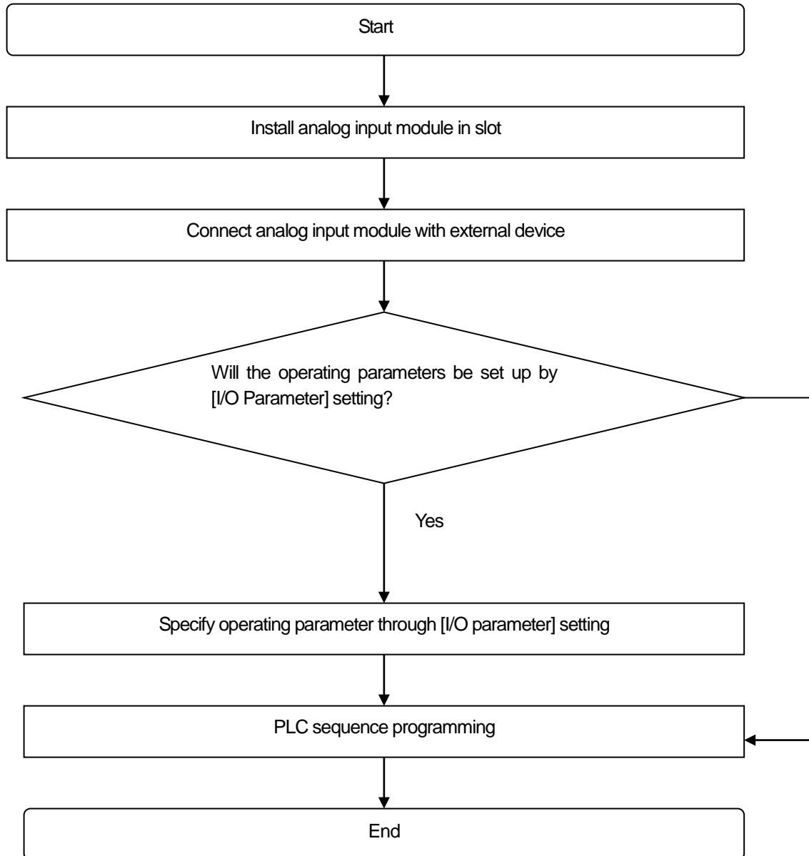
[Fig. 4. 1] Operating setting flowchart
