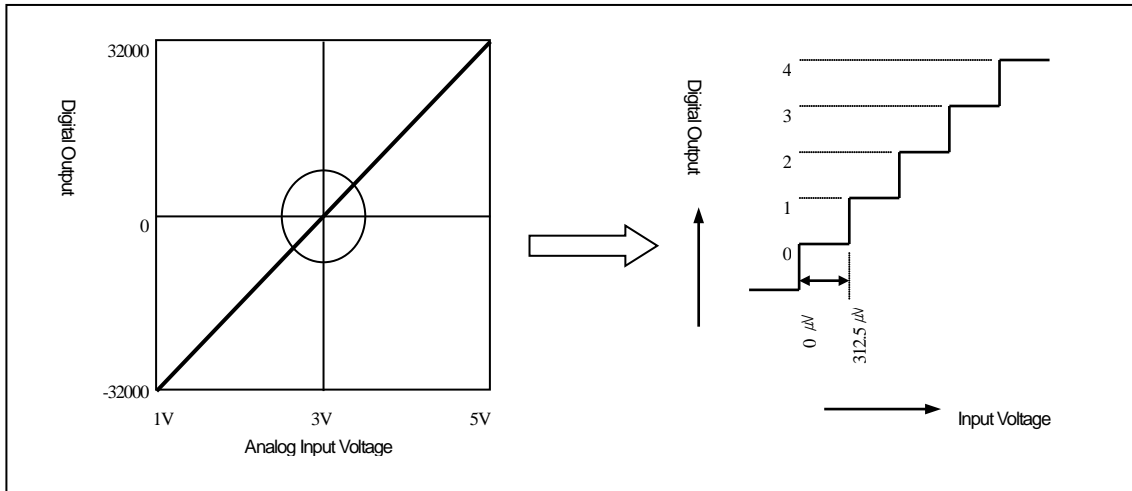
[Fig.1.5] A/D conversion characteristics (voltage input)
